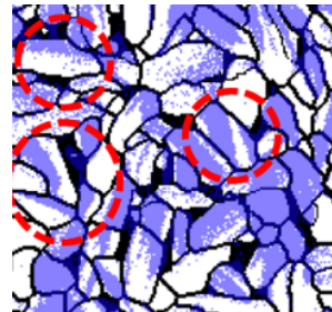
Fig 2: ferroelectric characterization of a 200-nm thick croconic acid film on ferromagnetic cobalt. (piezo-force microscopy). red dashed circles show some multi-domain grains. Area of \sim 1\mu\text{m} \times 1\mu\text{m} [moh20]
