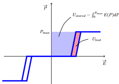
Fig1: energy storage principle on antiferroelectric with hysteresis
