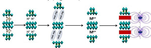
Figure 1. Schematic approach to the formation of 2D magnetic coordination networks in a confined layered environment.
