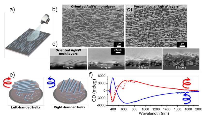
Fig. 1: a) Scheme of the Grazing Incidence Spraying (GIS) deposition, b) SEM image of a AgNW monolayer and c) of 2 perpendicular AgNW layers, d) cross-section SEM images of oriented AgNWs of varying thickness, e) scheme of chiral tri-layer samples, in which the director is rotated 60^\circ between each layer, and f) CD spectra, showing CD peaks of very high intensity for AgNWs (full) and AgNWs + an achiral dye (dashed).
